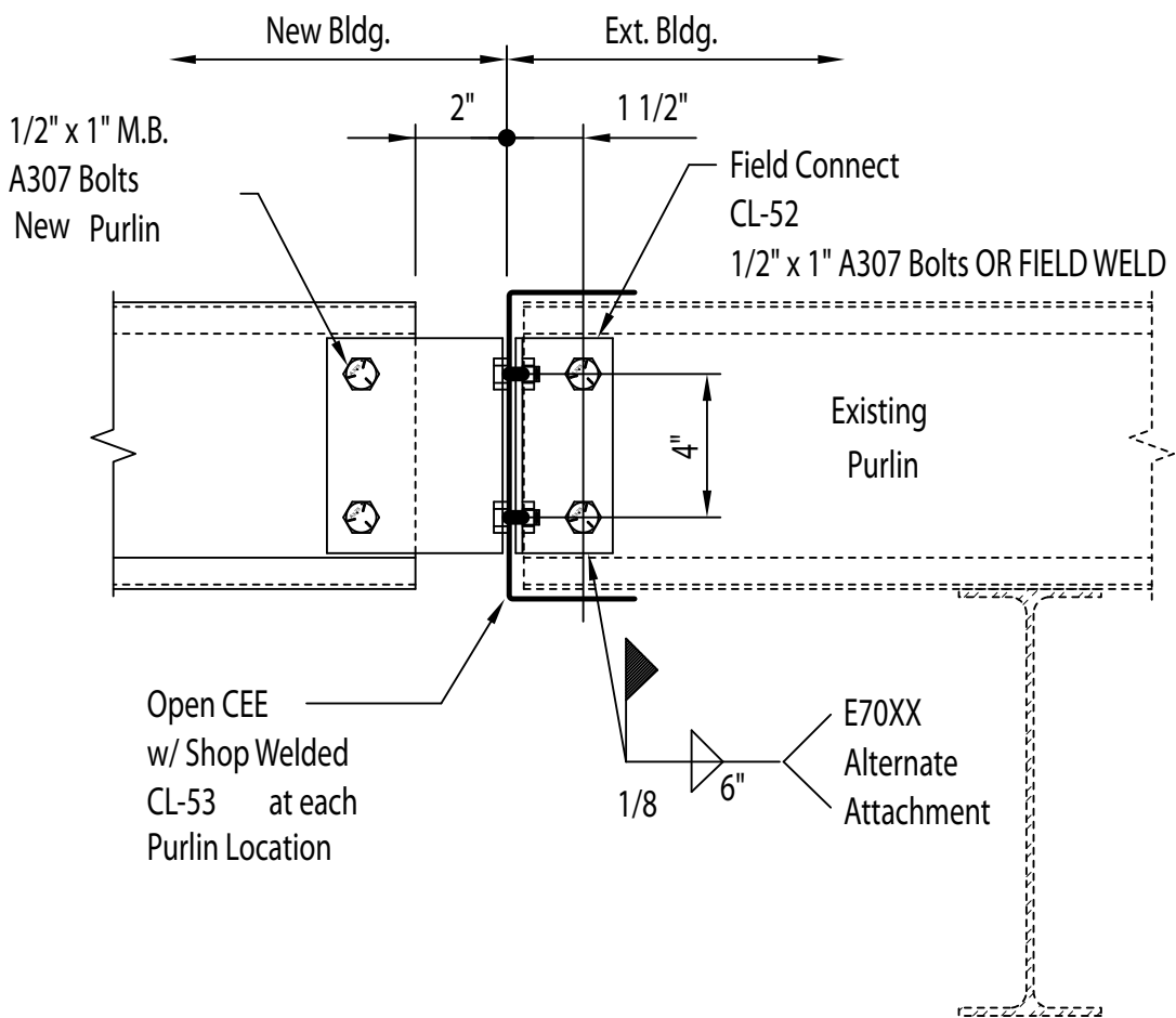
New To Old Purlin Tie-In Connection
