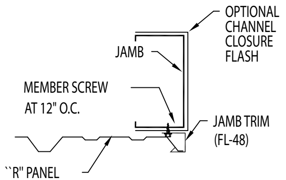
JAMB DETAIL FOR FRAMED OPENING ("R" PANEL)
