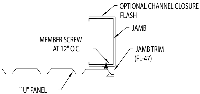
JAMB DETAIL FOR FRAMED OPENING ("U" PANEL)
