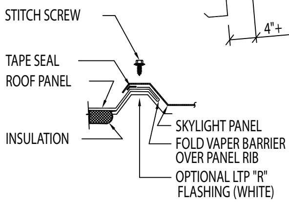
SIDE LAP WITH INSULATION
