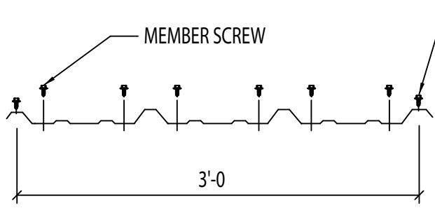
END LAP SCREW LAYOUT
