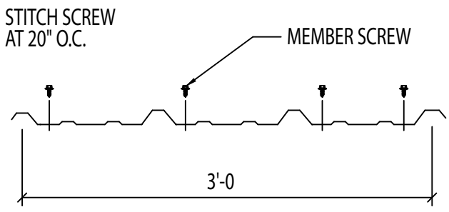
MID SPAN SCREW LAYOUT
